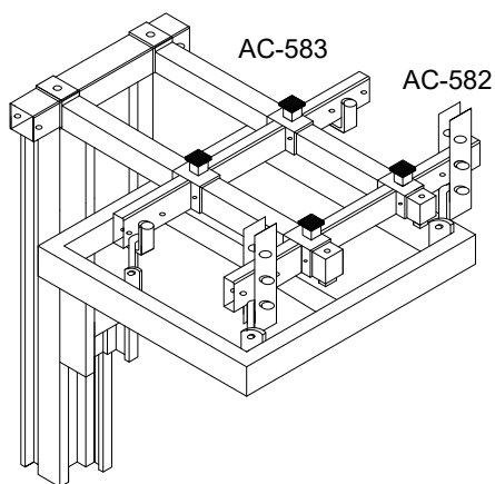
Hanging system 2
